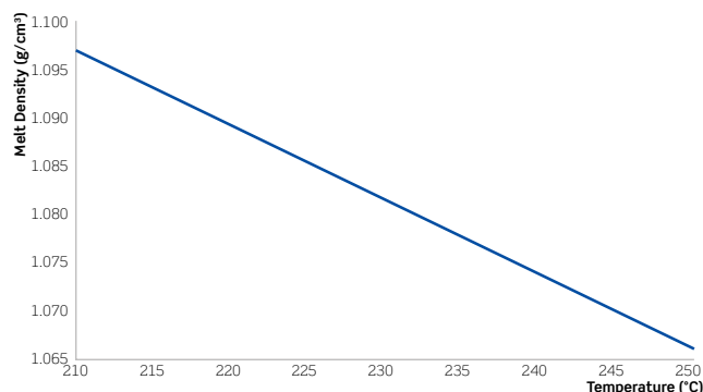
Figure 2: Melt Density as a function of temperature
