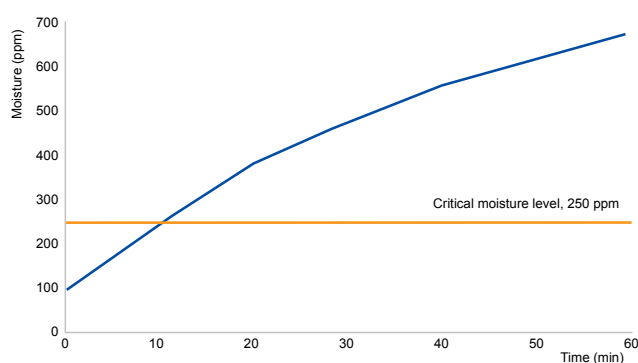
Figure 1: Moisture take-up curve semi-crystalline PLA
